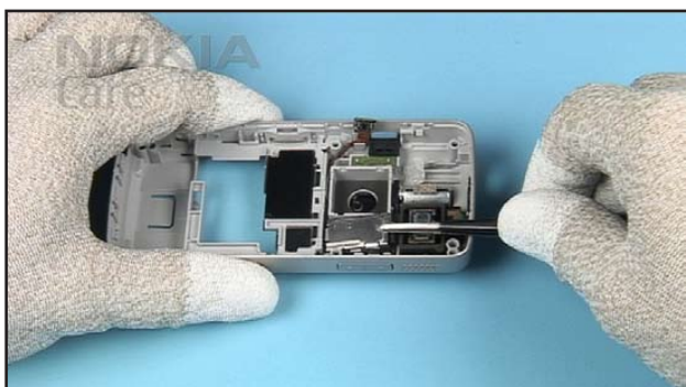
13. Place the FLASH HOLDER onto the FLASH...
