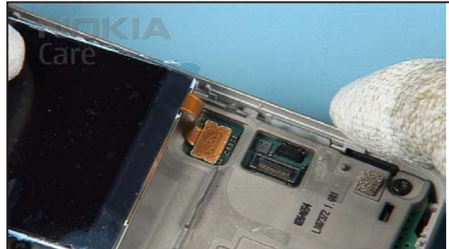
34. Place the LCD onto the MAIN FRAME paying attention to the LCD flex.
