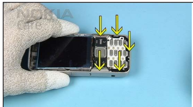
36. Fit the UI ASSY into the B-COVER.
