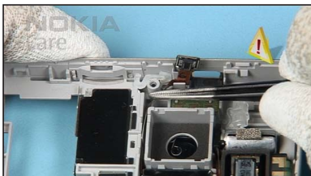
12. Check the correct position of the flex connector.
