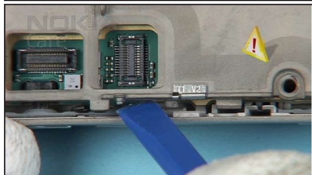
24. Open the snap on the other side.
