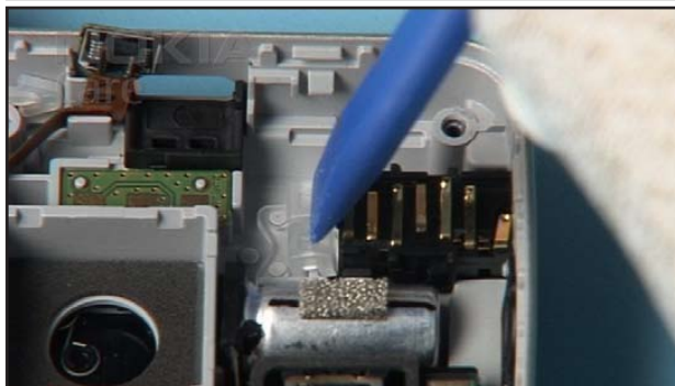
16. ...and secure it.
