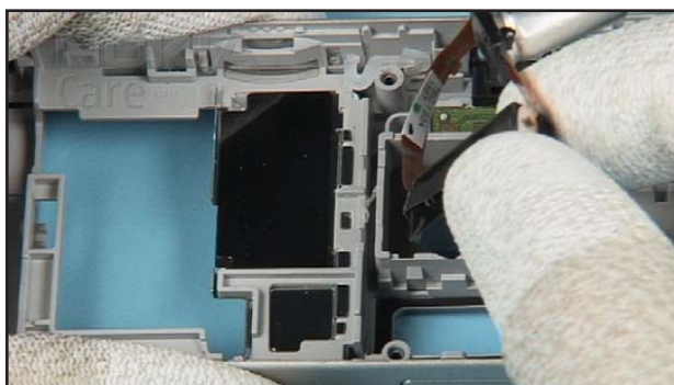
44. ...paying attention to the flex foil.
